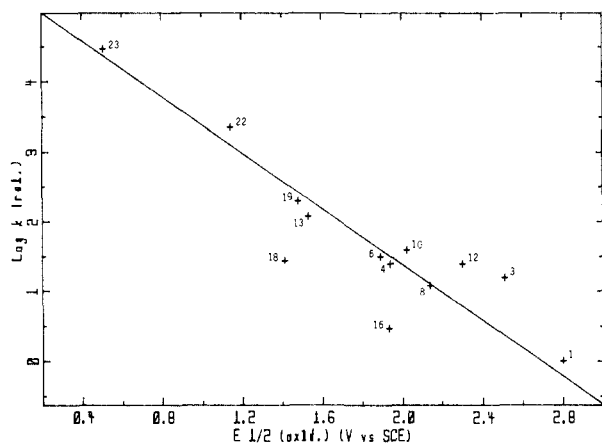
Figure 5. Correlation of \log k_{rel} for epoxidation of alkenes with the solution oxidation potentials of the alkenes as in Figure 4.
