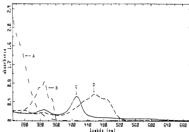
Figure 1. Spectra taken in CH 2 Cl 2 /CH 3 OH/H 2 O (80/18/2): pentafluoriodosylbenzene ( 5 \times 10^{-4} M) (A); trans,trans -1,4-diphenylbutadiene ( 10^{-5} M) (B); [tetrakis(2,6-dichlorophenyl)porphyrin]iron(III) chloride ( 4 \times 10^{-6} M) (C); \beta -carotene ( 3 \times 10^{-6} M) (D).
