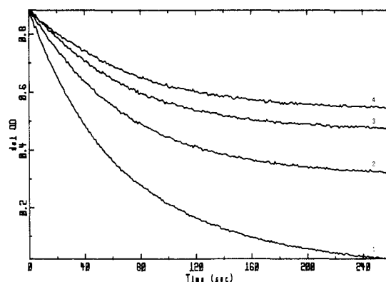
Figure 2. Plots of absorbance ( \Delta\text{OD} at 348 nm) vs time for competitive epoxidation of 1,4-diphenylbutadiene ( C_1 ) and cis -2- trans -4-hexadiene ( C_2 ) with PFIB ( C_3 ) at 10^{-6} M in hemin I. Concentrations ( M \times 10^5 ): 1, [ C_1 ] = 3.03, [ C_2 ] = 0, [ C_3 ] = 2.7; 2, [ C_1 ] = 2.95, [ C_2 ] = 17.1, [ C_3 ] = 2.63; 3, [ C_1 ] = 2.94, [ C_2 ] = 22.1, [ C_3 ] = 2.62; 4, [ C_1 ] = 2.92, [ C_2 ] = 25.4, [ C_3 ] = 2.61.
