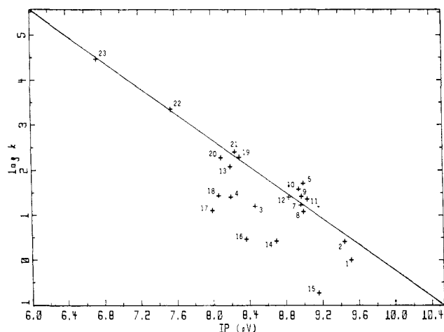
Figure 4. Correlation of \log k_{rel} for epoxidation with vertical ionization potentials of the alkene. Numbers identify the alkenes of Table I.
