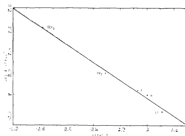
Figure 6. Correlation of \log k_{rel} for hemin I catalyzed epoxidation of para-substituted styrenes with \sigma_p^+ for the substituent.
